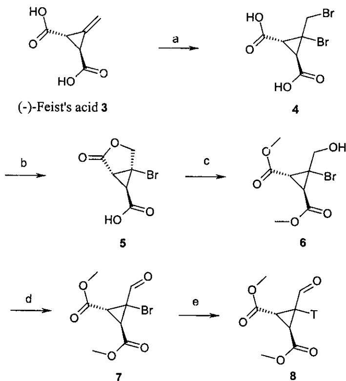
Scheme 1. Synthesis of 8 . a) Br 2 in diethyl ether, RT, 16 h, 64%; b) H 2 O, reflux, 4 h, 61%; c) MeOH, conc. sulfuric acid, RT, 2 h, 97%; d) PCC, MeCl 2 , RT, 16 h, 69%; e) Bu 3 SnT, AIBN, cyclohexane-THF, 50°C, 18 h.
